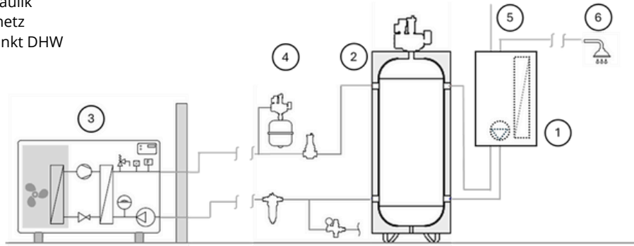
KONDENSATIONSKESSEL-SCHEMA
