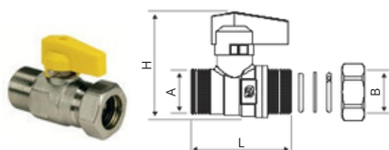
ART. 1223 M x OLIVE
