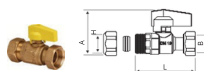
ART. 1225 OLIVE x F
