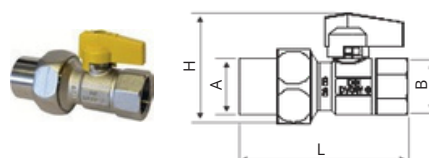
ART. 1481 F x F
