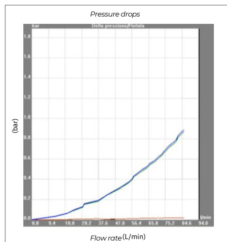
HEATING PRESSURE DROPS
