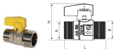
ART. 1221/B M x M
